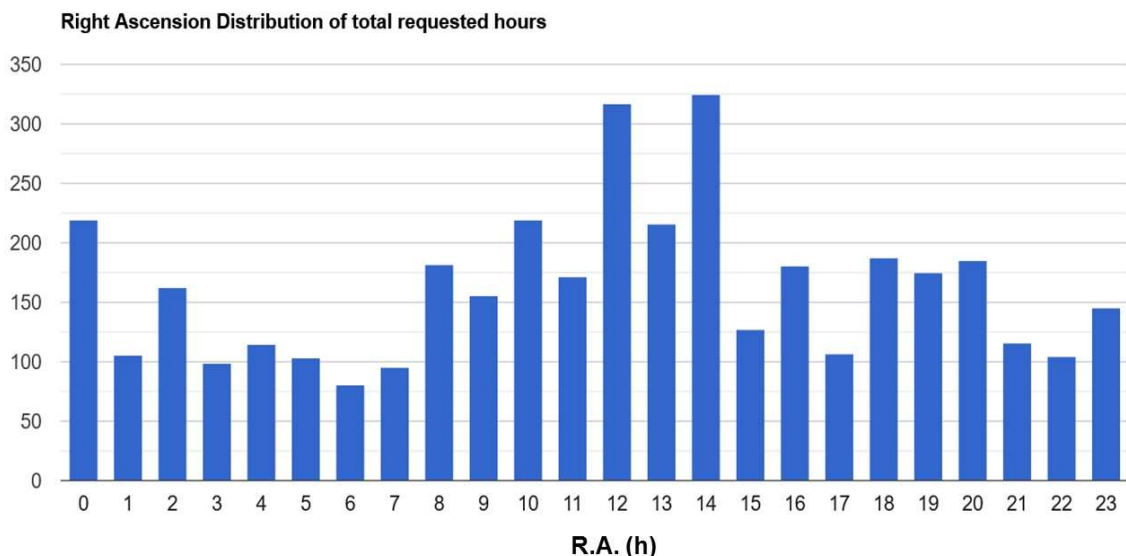
Figure 1: R.A. distribution for OBs that were requested to be executed in S21B+S22A. Note the high oversubscription in RA=12-14h and the relatively low demand for RA=19-23h.
